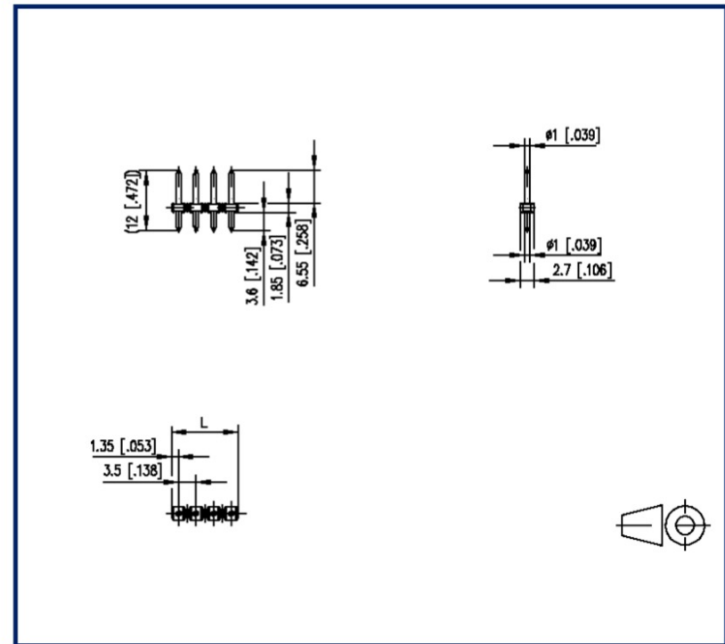
Dimensional drawing as an example
